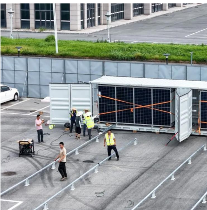
Bluesun 20FT Container Solar System 250KW 860KWH ...
